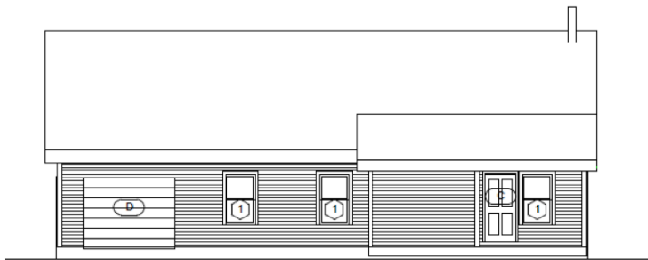
① EAST ELEVATION 1/8" = 1'-0"
