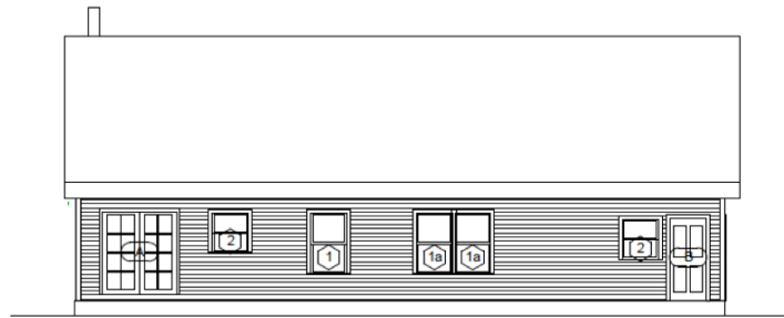
③ WEST ELEVATION 1/8" = 1'-0"
