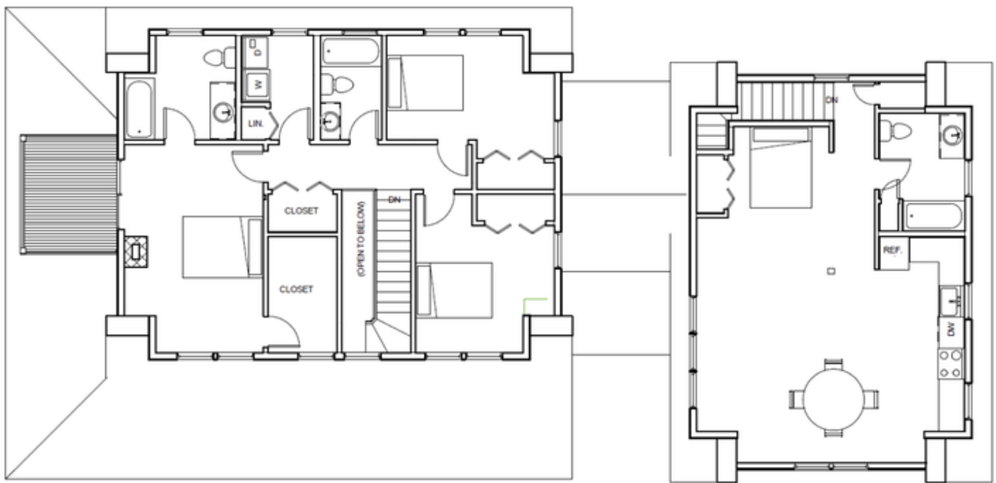
① LEVEL 3 3/16" = 1'-0"
