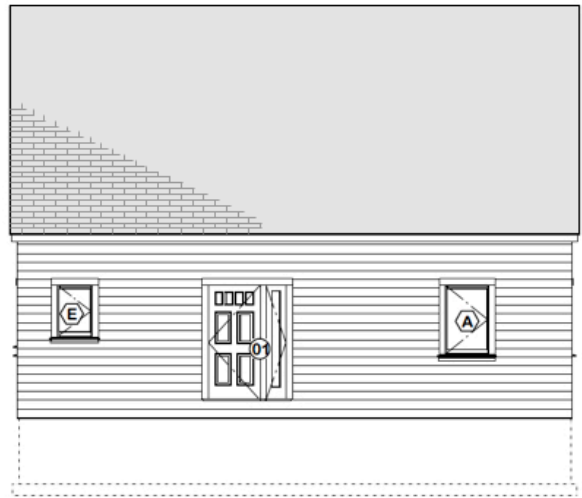
1 FRONT ELEVATION scale 1/4 inch = one foot
